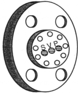
Pneumatic Flange Mount Diaphragm Level Sensor #ILS-2113
